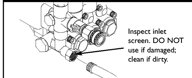
Figure 3 — Connect Garden Hose to Water Inlet
